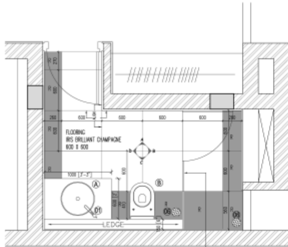
BATHROOM 2 9'-0" x 6'-0"
